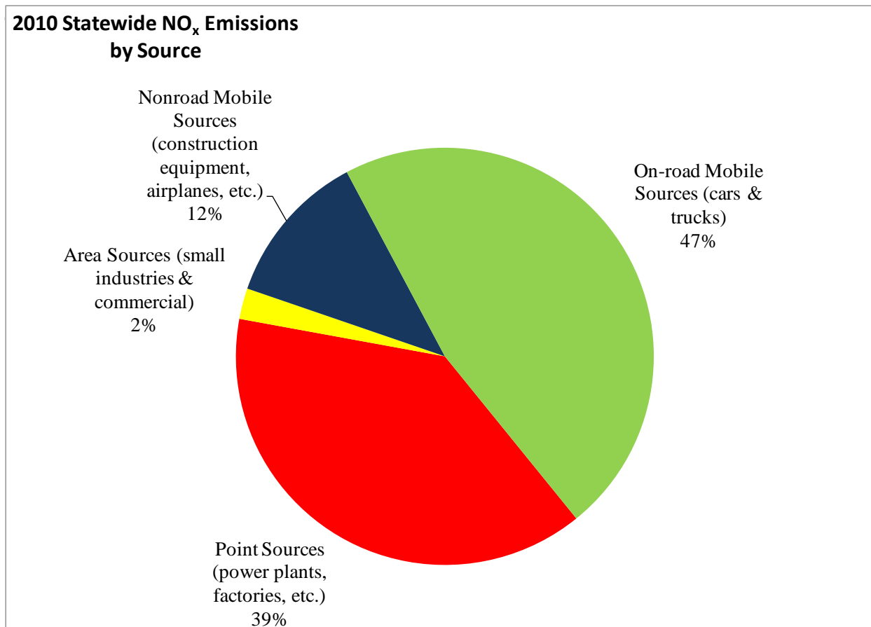
Figure 1. 2010 statewide NO x emissions by source category.
